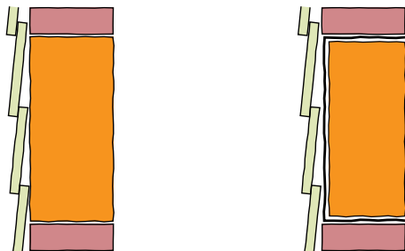
a) Without cavity and without underlay. b) Without cavity and with a new underlay.
