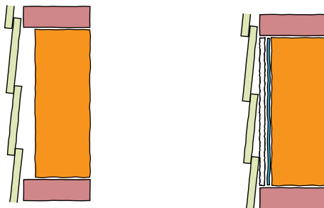
c) With 20 mm separation between insulation and cladding and without underlay. d) With drainage plane mesh and new underlay.
